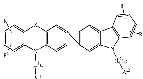
Chemical Formula 4
