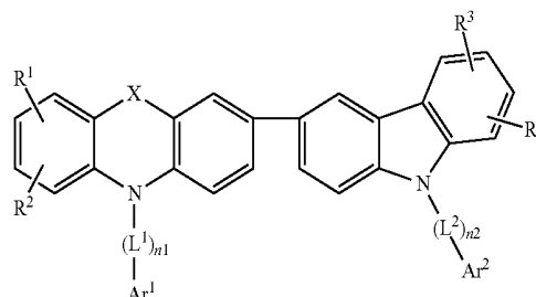
Chemical Formula 2
