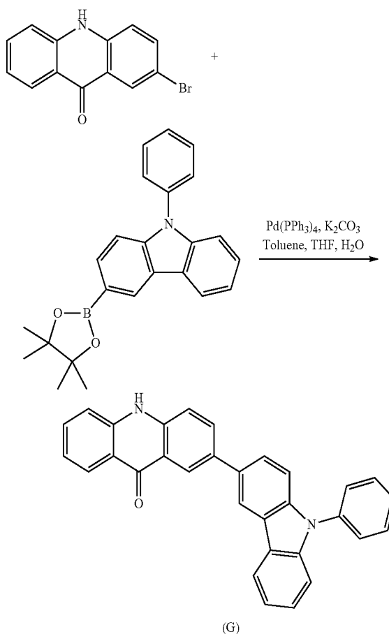
Reaction Scheme 7
