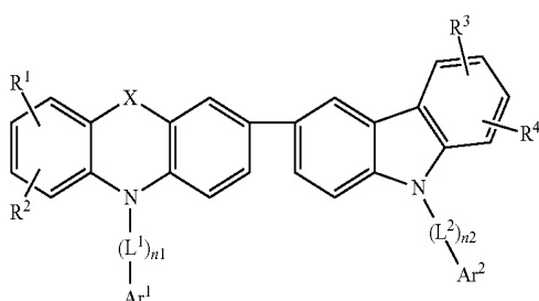
Chemical Formula 2
