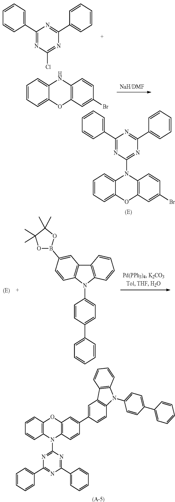
Reaction Scheme 5
