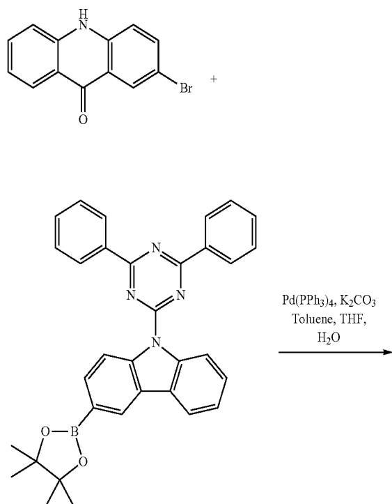
Reaction Scheme 4
