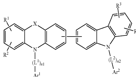
Chemical Formula 1
