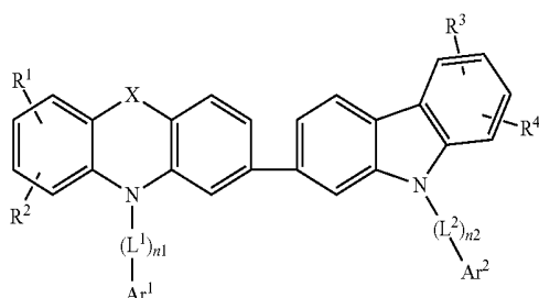
Chemical Formula 3
