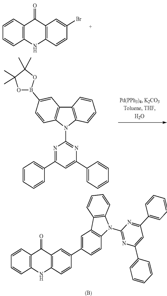
Reaction Scheme 2
