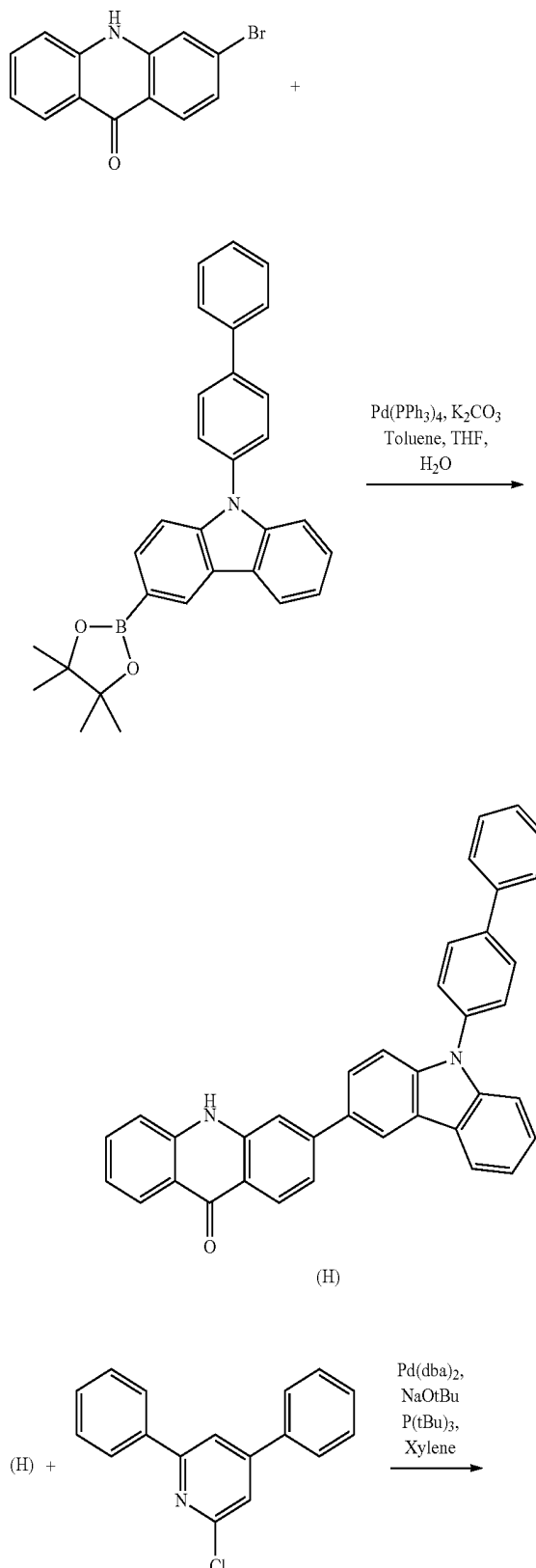
Reaction Scheme 8
