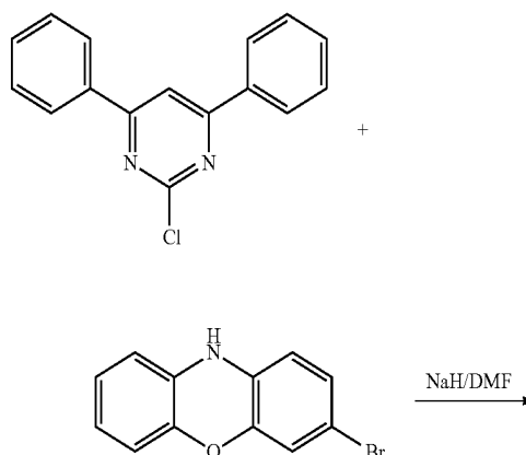
Reaction Scheme 6
