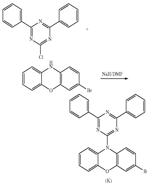
Reaction Scheme 11
