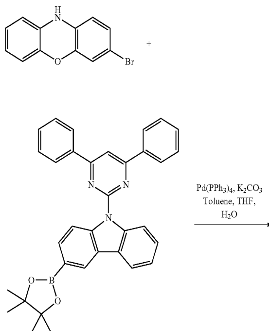
Reaction Scheme 10
